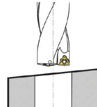
2. Drilling on inclined surface
