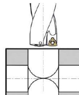
3. Cross-hole drilling
