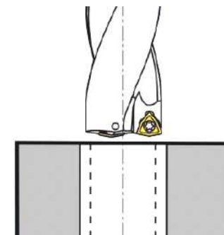
4. Expand drilling
